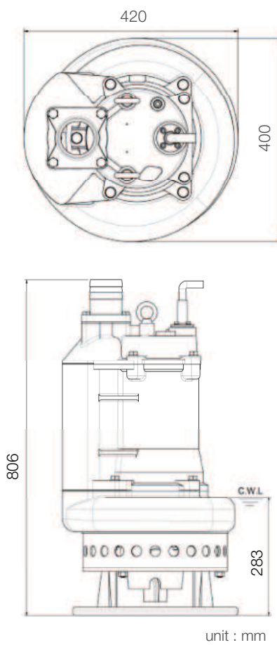
Opened Impeller
